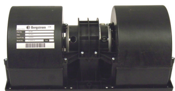
Bluebird Blower Assembly (New Style) fits Visions and others Part# 1099097 Cross Ref #'s 519703, BFZ80, 00090195
